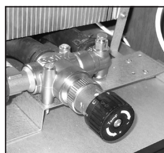
Shunt valve for floor heating (certain motorhomes only).
