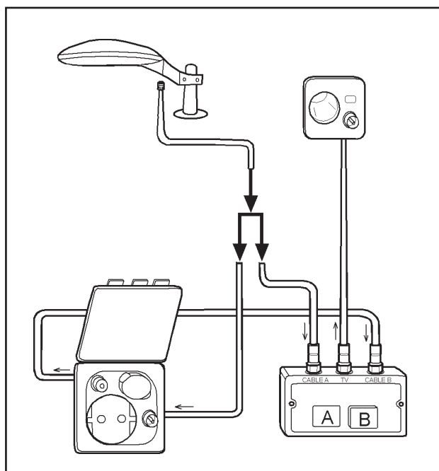
Schematic of the motorhome's antenna system.
