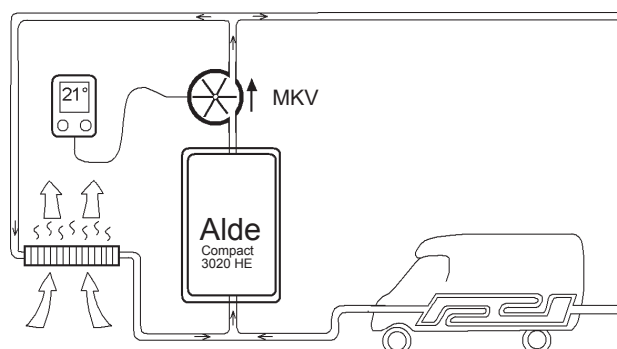
Figure 1: Schematic of the living area's heating system.
