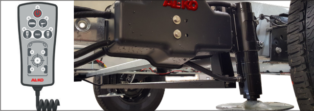
AL-KO HY4 hydraulic support legs. Simply press the button on the controller to level your vehicle. To activate night mode with a slight inclination forward, just press that button. Yet another button will pull in the support legs entirely. You can also manage HY4 manually and control combinations of support leg pairs as you wish. Each leg has its own motor and the entire system is mounted on the chassis. Not inside the vehicle. HY4 is standard in Imperial, available as an option in others.
