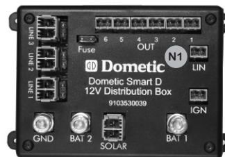
Elsystemets enhed N1. Dometic Smart D 12V Distribution Box.
